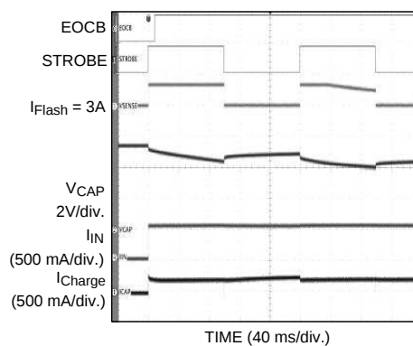
Figure 31. Level-Sensitive Strobe
