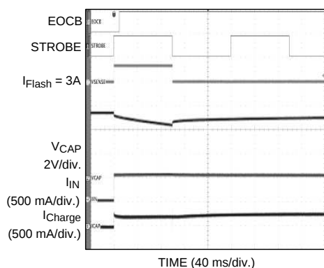
Figure 30. Edge-Sensitive Strobe
