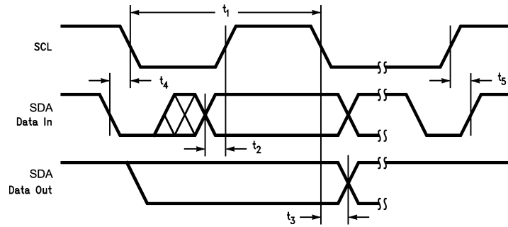
Figure 1. LM3550 Timing
