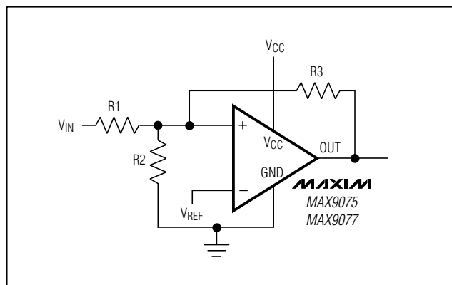
Figure 1. Adding Hysteresis
