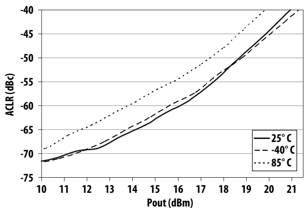
Figure 67. ACLR (Dual Carrier Signal) vs Pout at 2650 MHz
