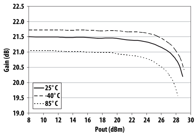
Figure 65. Gain vs Pout at 2650 MHz
