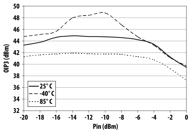
Figure 66. OIP3 vs Pin at 2650 MHz
