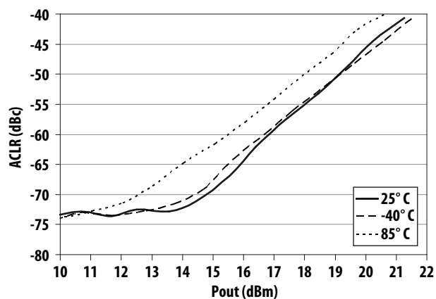
Figure 68. ACLR (Single Carrier Signal) vs Pout at 2650 MHz
