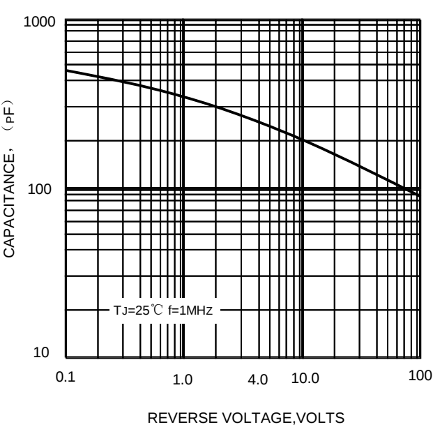
FIG.4-TYPICAL JUNCTION CAPACITANCE
