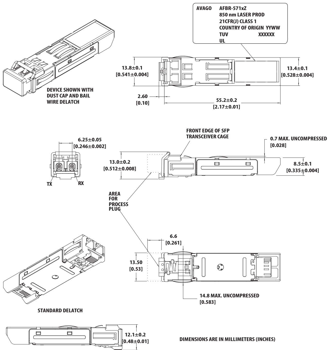
Figure 7. Module drawing
