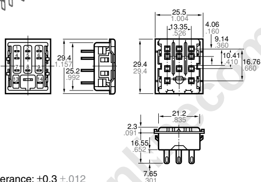
External dimensions
