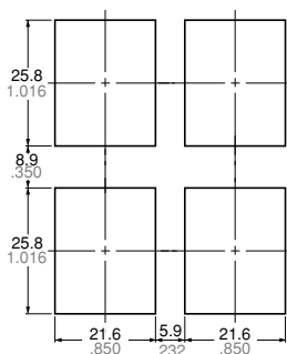
Side-by-side installation
