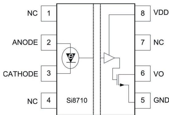
Figure 12. Pin Configuration
