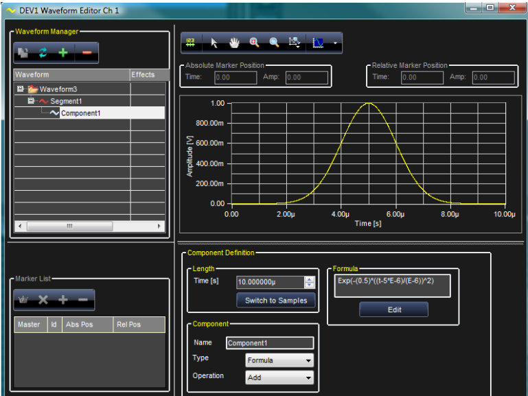
A Gaussian pulse waveform. The actual formula used here is \text{Exp}(-(0.5)*((t-5*\text{E}-6)/(E-6))^2) . Set the time to 10.000000μ to view the graph as previously shown.
