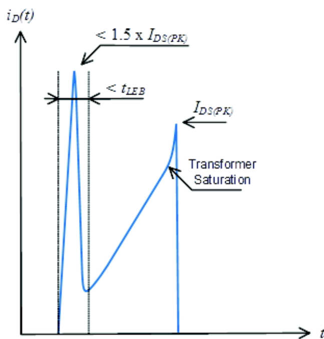
Figure 3. Spike Limits
