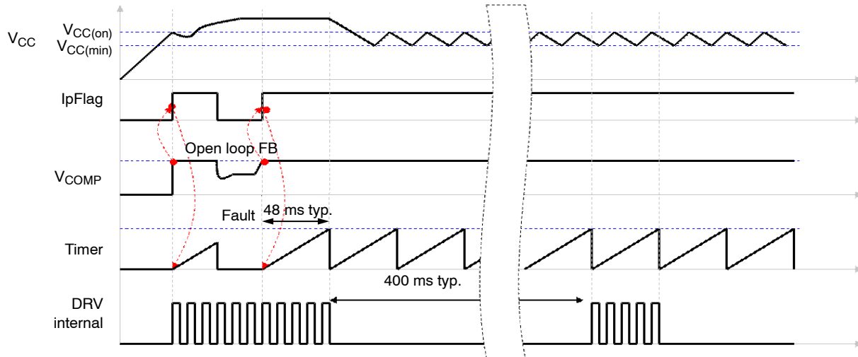
Figure 33. In Case of Short-circuit or Overload, the NCP106X Protects Itself and the Power Supply via a Low Frequency Burst Mode. The V_{CC} is Maintained by the Current Source and Self-supplies the Controller
