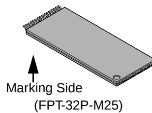
32-pin plastic TSOP (I)
