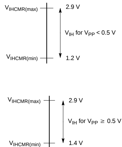
Figure 14. MC100LVEL14 Common Mode Range
