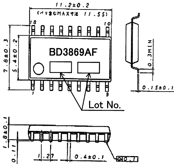
SOP-18 (Unit : mm)
