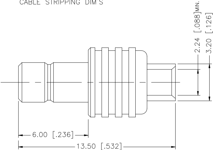
RECOMMENDED CABLE STRIPPING DIM'S
