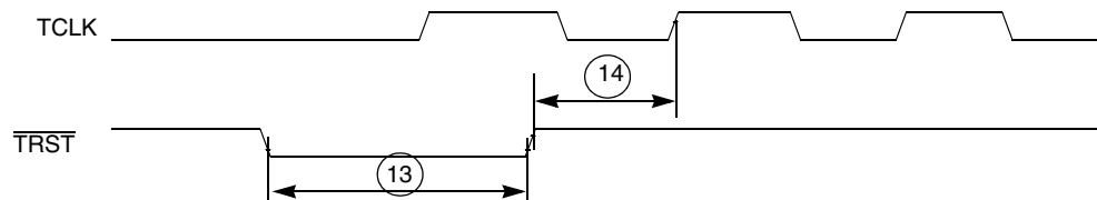
Figure 17. TRST Timing
