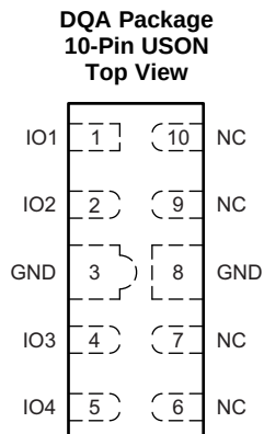
Pin Functions
