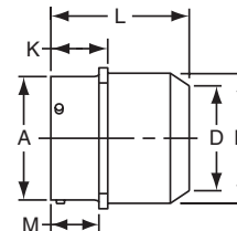
“CP” Potting Boot
