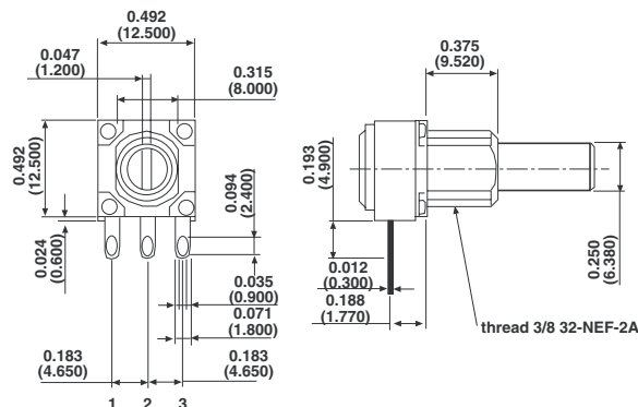
SOLDER LUG TERMINALS
