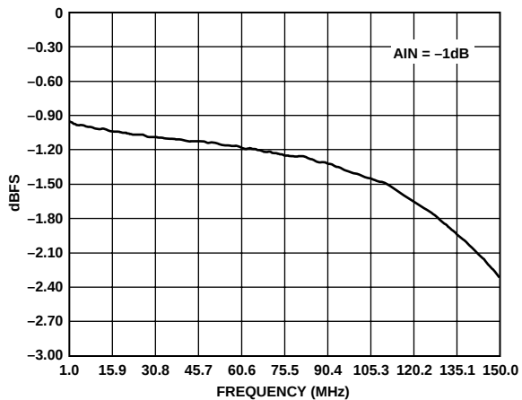
Figure 14. Gain Flatness
