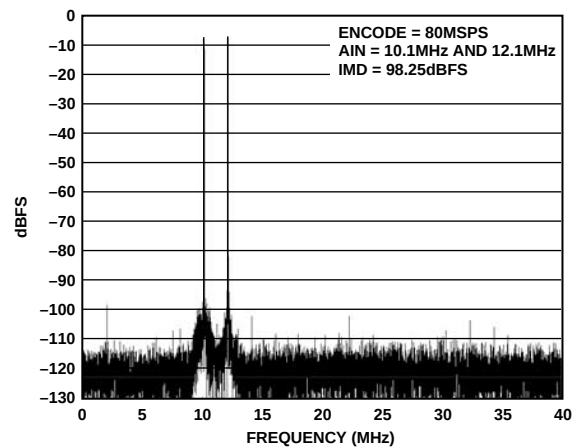
Figure 12. Two-Tone at 10.1 MHz and 12.1 MHz
