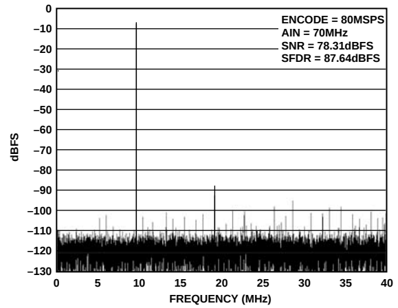
Figure 11. Single-Tone at 70 MHz
