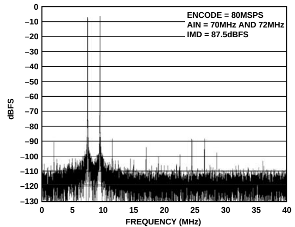
Figure 13. Two-Tone at 70 MHz and 72 MHz
