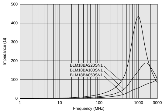
BLM18BA Series (50ohm to 220ohm)
