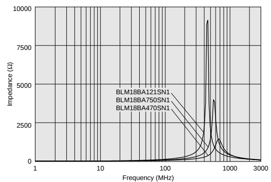
BLM18BA Series (470ohm to 120ohm)
