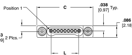
Plug with Flying Leads Drawing Number 1589455
