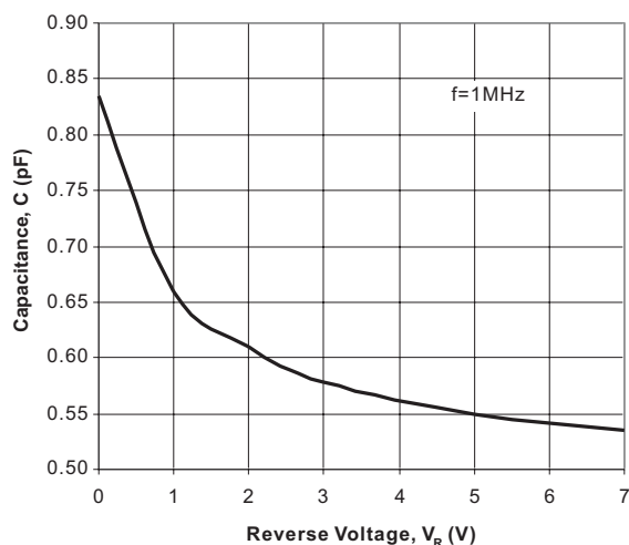
FIG. 3 TYPICAL TOTAL CAPACITANCE
