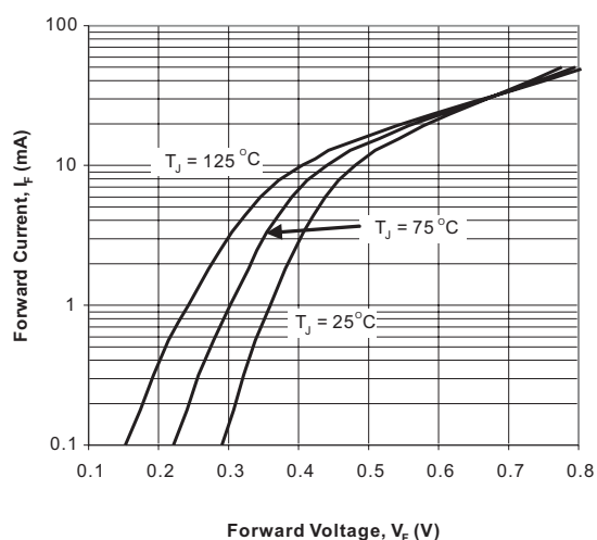
FIG. 1-TYPICAL FORWARD CHARACTERISTIC
