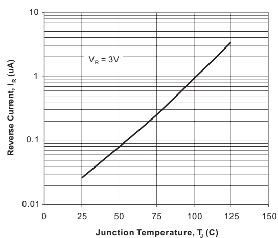
FIG. 2-TYPICAL REVERSE CHARACTERISTICS
