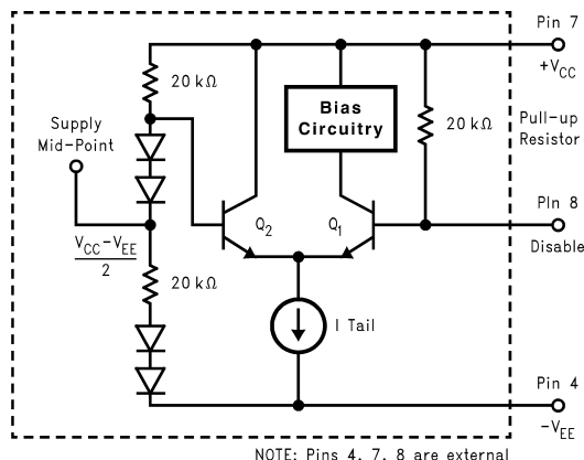
Figure 34. Enable/Disable Operation
