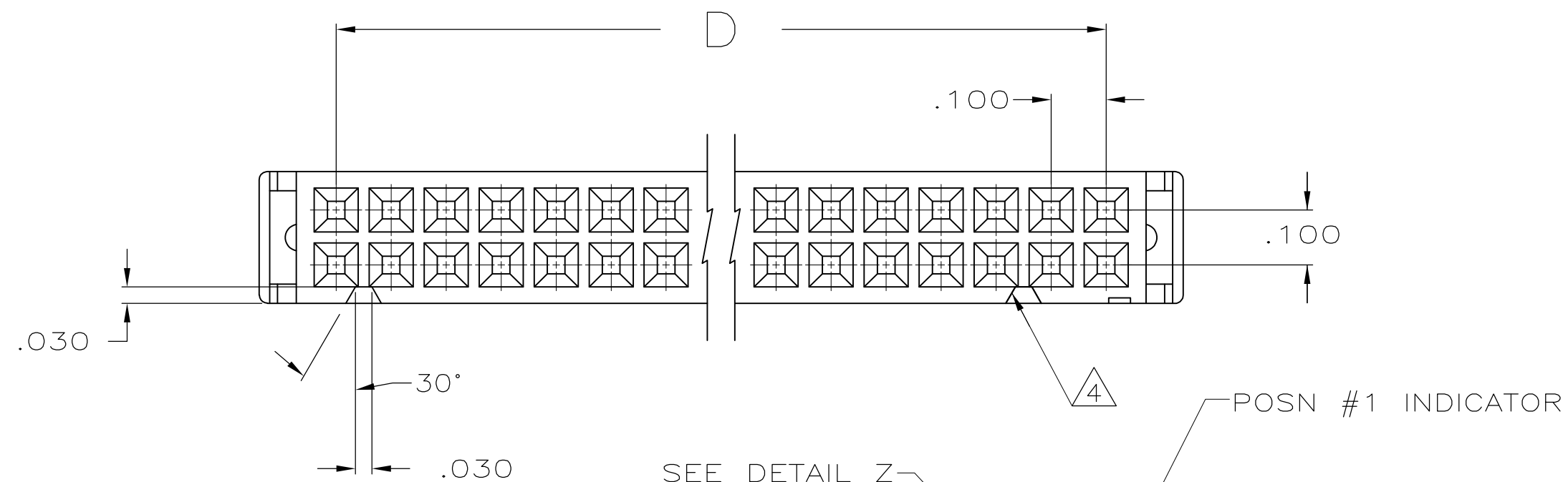
TERMINATED VIEW
