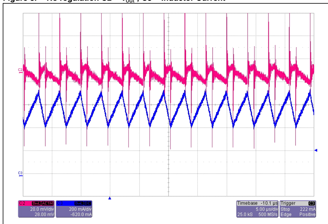
Figure 8. No regulation C2 = V_{\text{out}} ; C3 = Inductor Current
