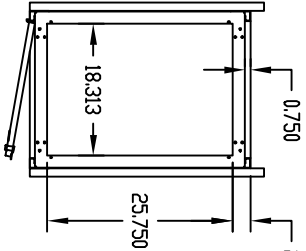
TOP VIEW (LESS TOP COVER & FRONT TOP TRIM)
