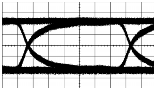
Output Waveform
