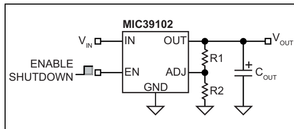
FIGURE 4-2: Adjustable Regulator with Resistors.
