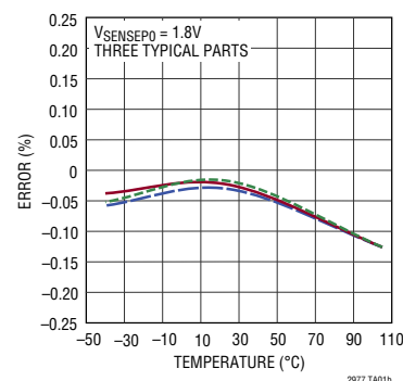
Typical ADC Total Unadjusted Error vs Temperature
