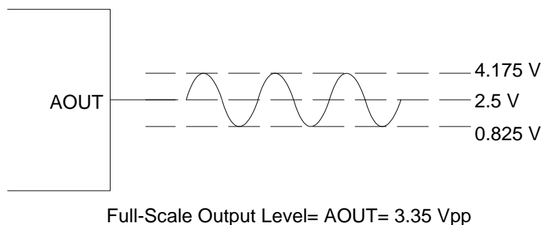
Figure 19. Full-Scale Output
