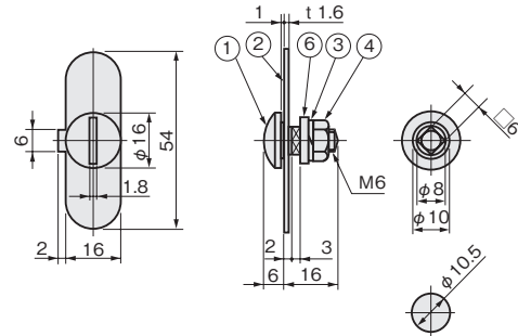
Layout of Holes for Installation
