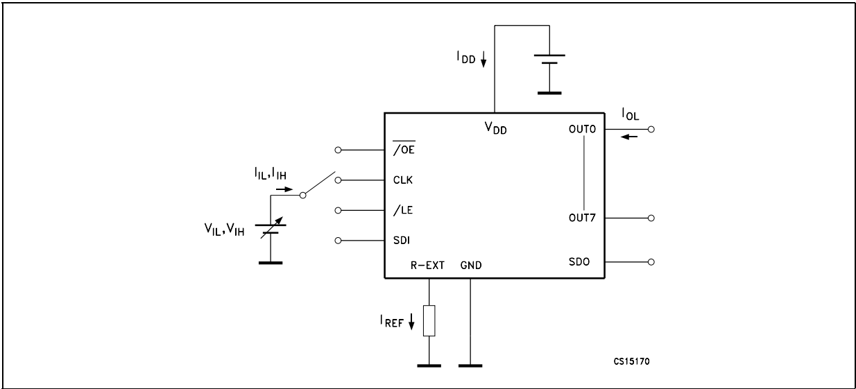
Figure 11: DC Characteristic
