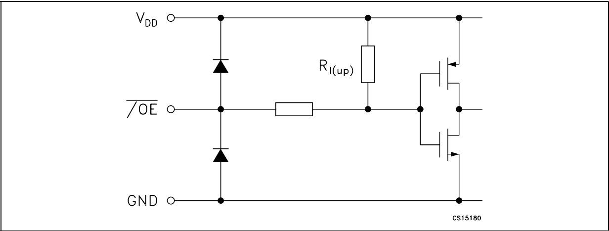
Figure 2: \overline{\text{OE}} Terminal
