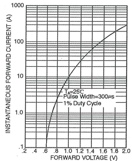
FIG. 3 - TYPICAL FORWARD SURGE CURRENT
