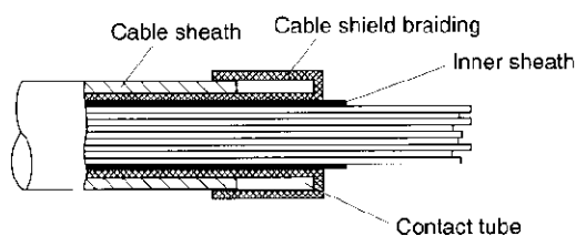
Mounting method B (preferred)
