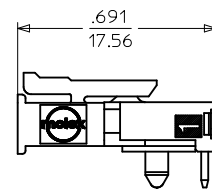
MATED MICRO FIT CONNECTOR
