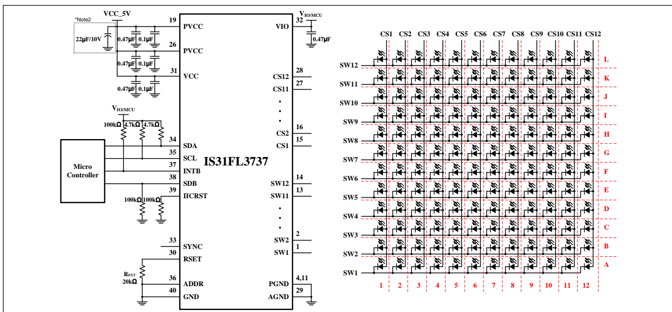
Figure 1 Typical Application Circuit (12x12)
