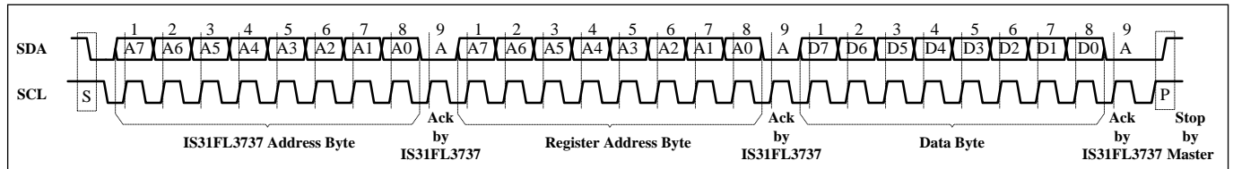
Figure 6 Writing to IS31FL3737 (Typical)
