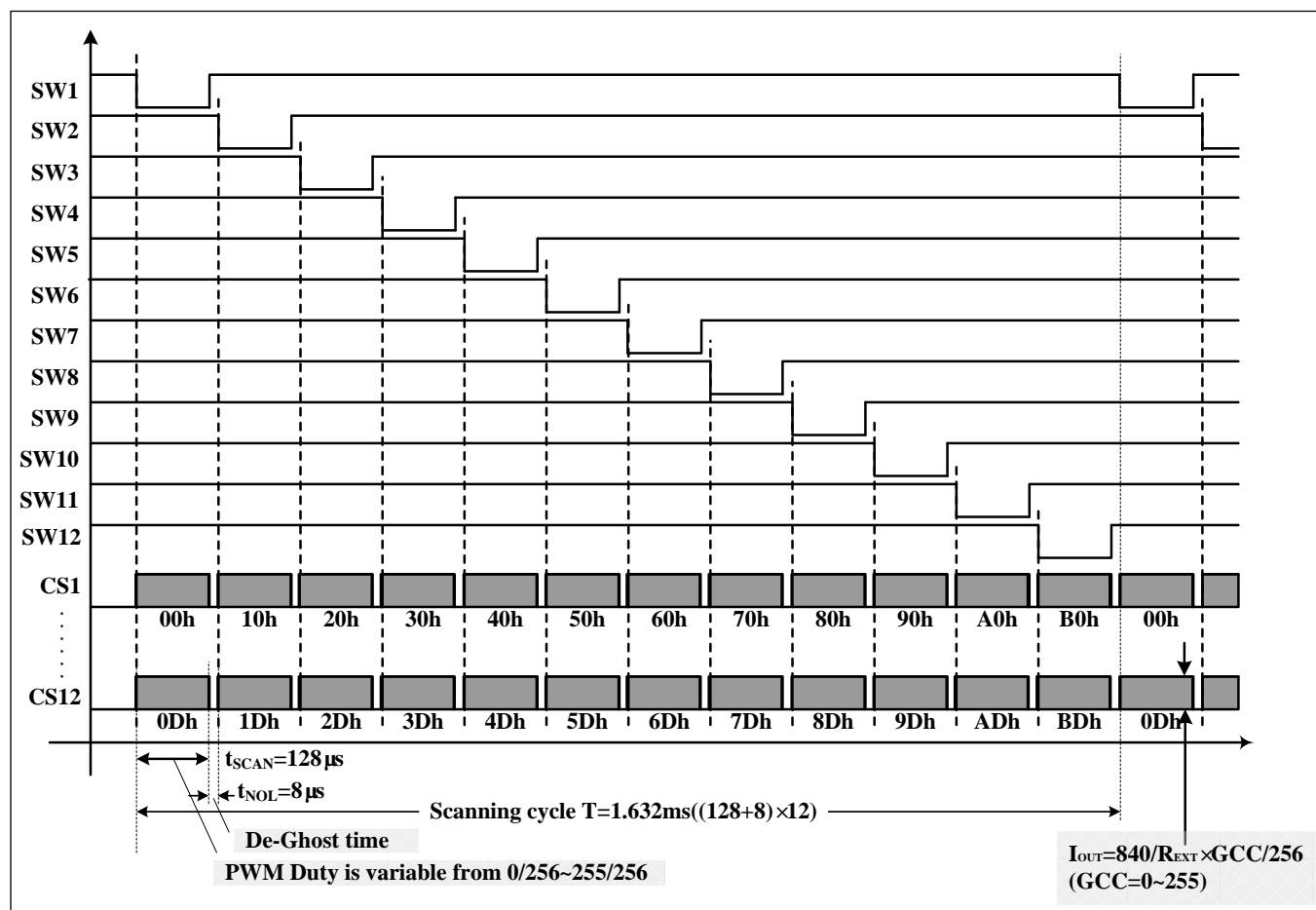
Figure 12 Scanning Timing
