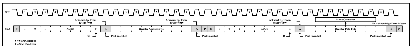
Figure 8 Reading from IS31FL3737
