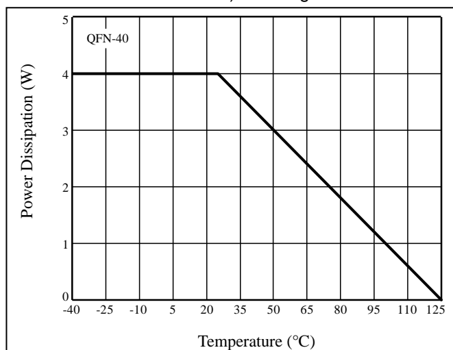
Figure 17 Dissipation Curve
