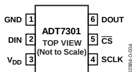
Figure 4. SOT-23
