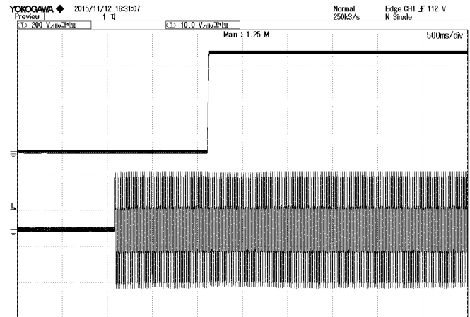
Figure 5: Vout start up at 220Vac, 10.5A Iout, TOP: Vin, 200V/div, 500ms/div BOTTOM: VOUT, 10V/div, 500ms/div
