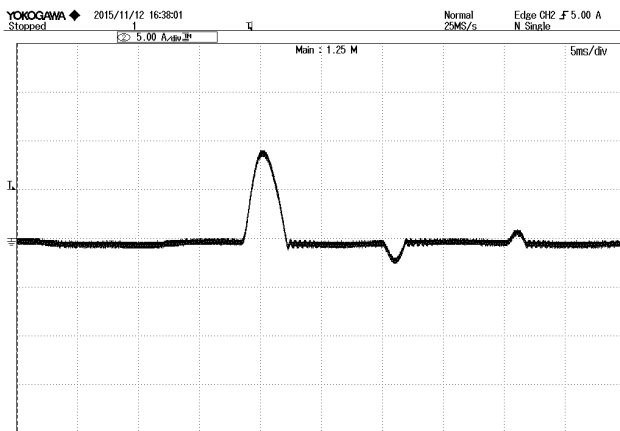
Figure 6: Output ripple & noise at 220Vac, 10.5A Iout VOUT: 100mV/div, 10ms/div
