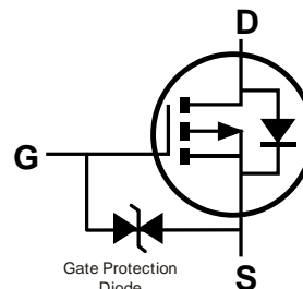
Equivalent Circuit
