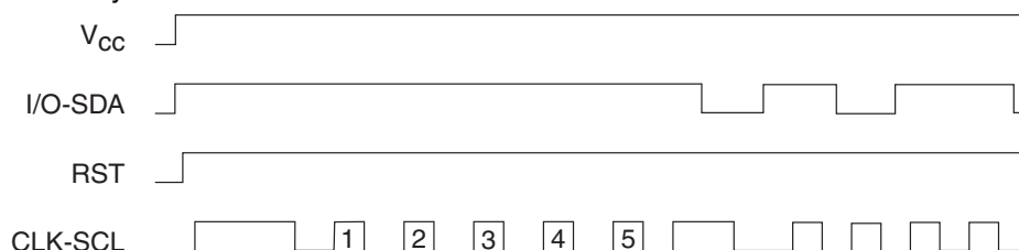
Figure 3. Synchronous 2-wire Protocol
