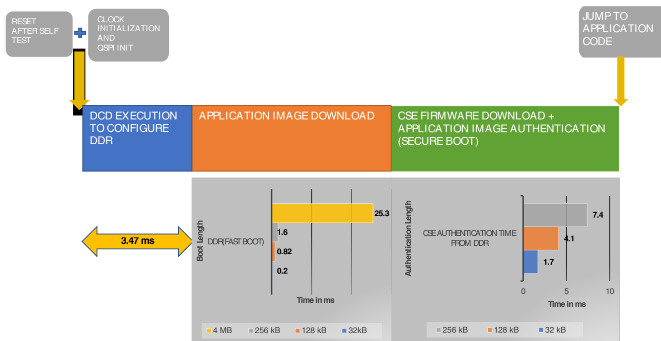
Figure 58. Boot diagram
