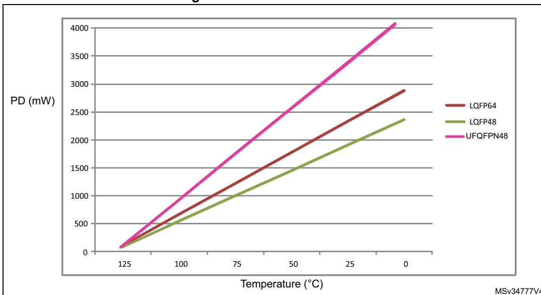
Figure 43. Thermal resistance
