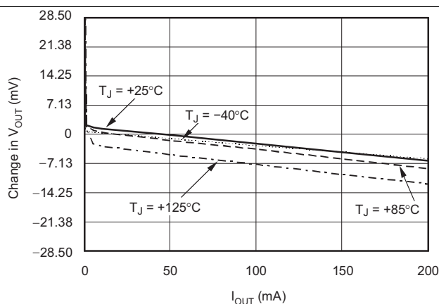
Figure 1. Load Regulation
