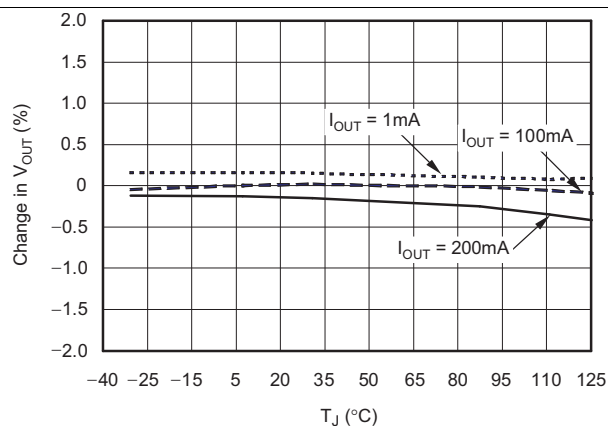
Figure 1. Load Regulation
