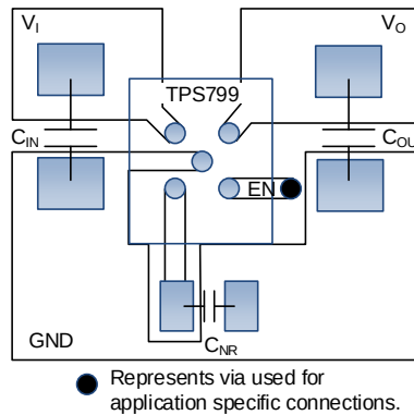
Figure 15. Layout Example
