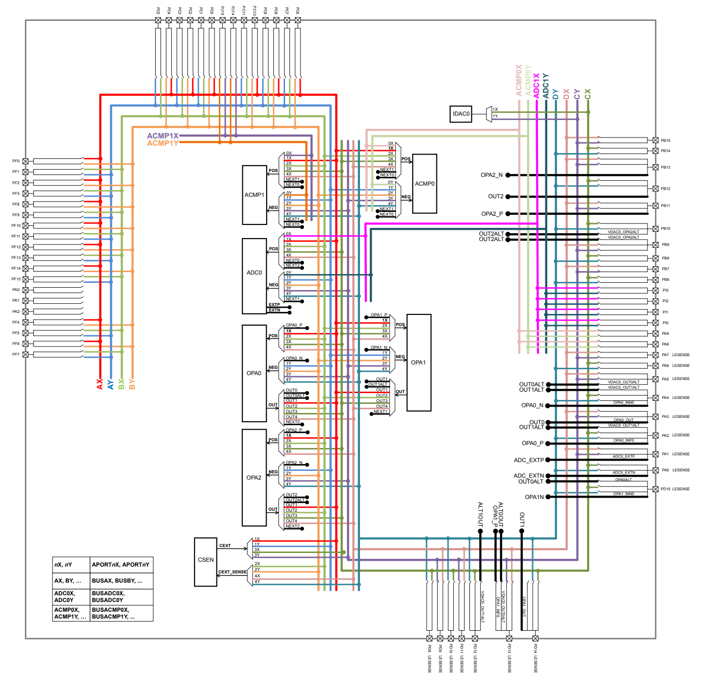
Figure 6.5. APORT Connection Diagram
