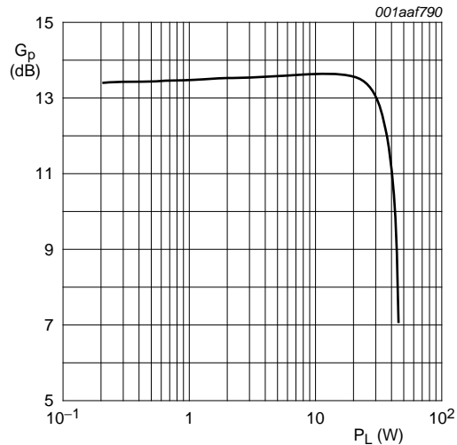
Fig 1. Power gain as function of CW load power; typical values
