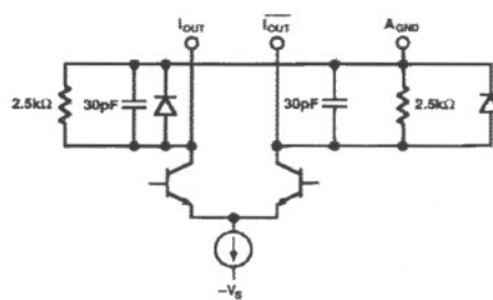
Output Circuit
