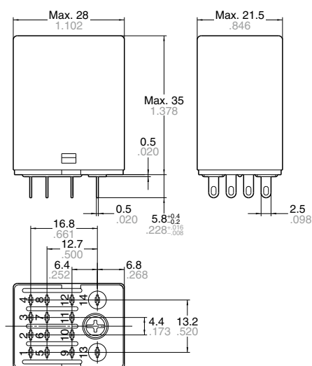
External dimensions
