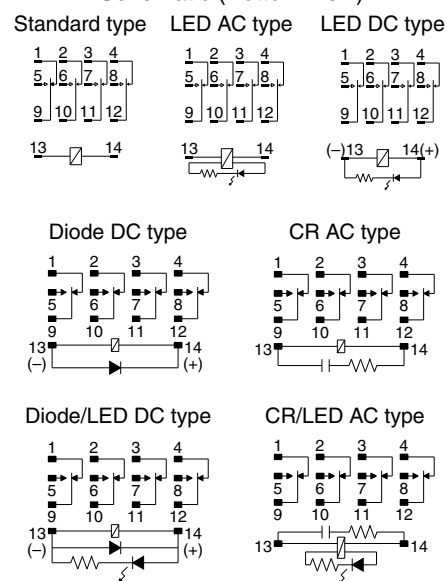
Schematic (Bottom view)
