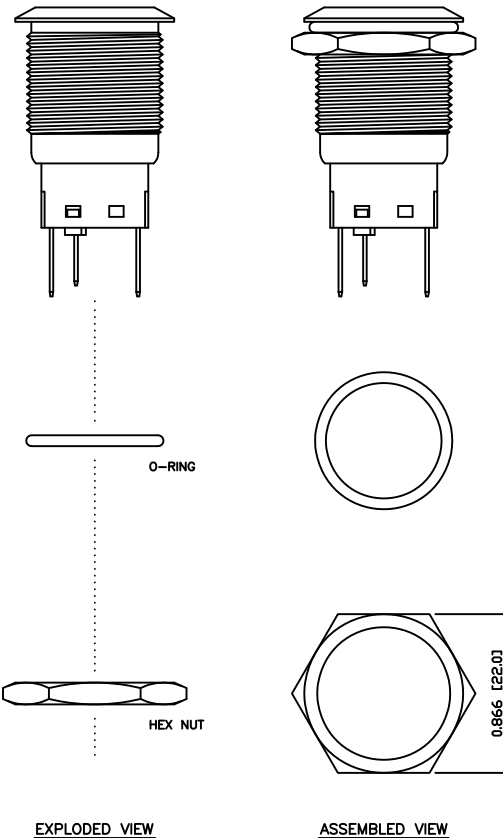
EXPLODED VIEW
