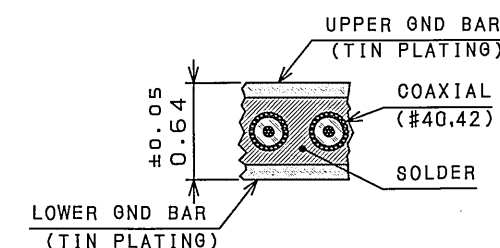
SECT. A-A
