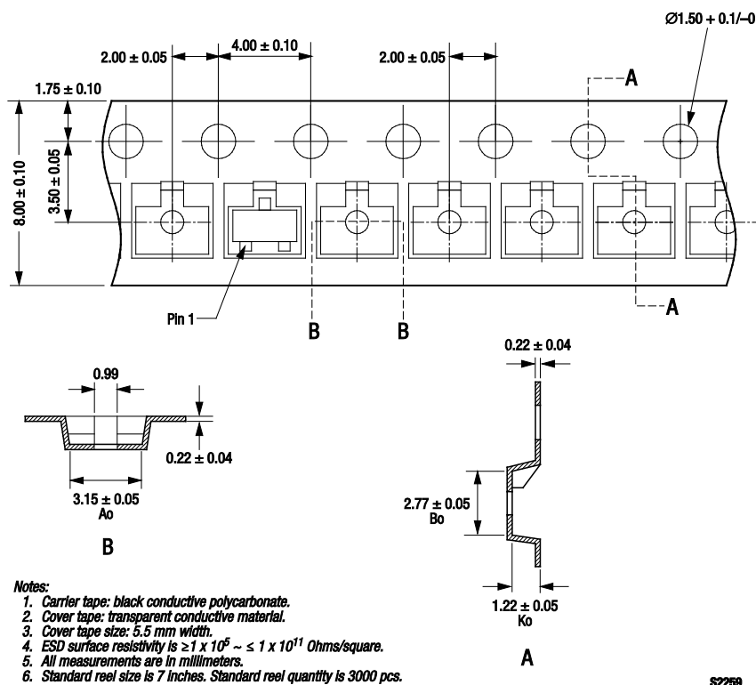
Figure 13. SOT-23 Tape and Reel Dimensions
