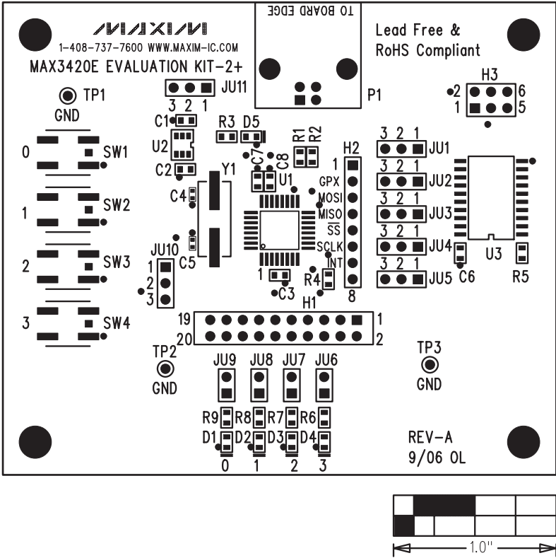
Figure 4. MAX3420E EV Kit-2 Component Placement Guide—Component Side
